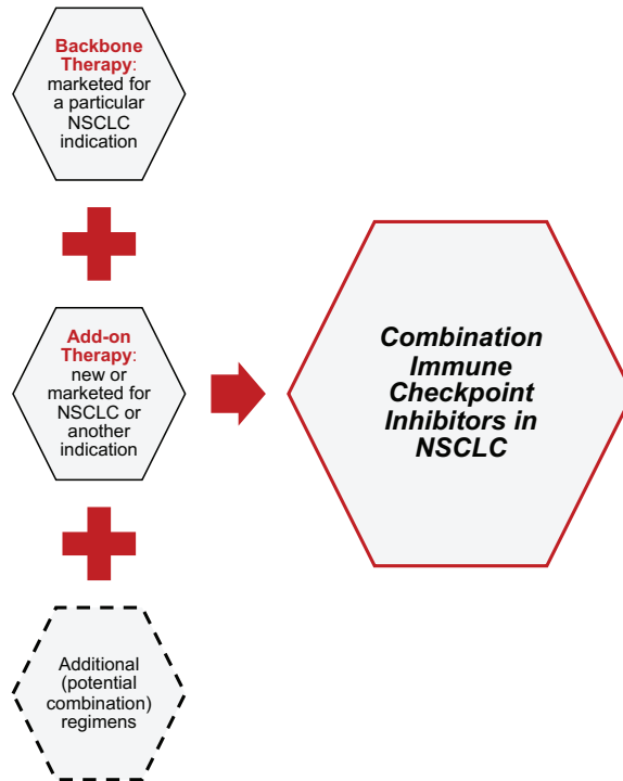
Figure 1. Legend A schematic representation of the constituents of a combination immune checkpoint inhibitor, including a backbone therapy, an add-on therapy, and (potential) additional drugs.
